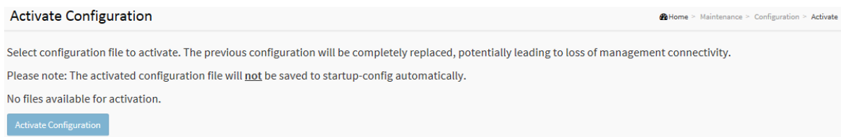
Figure 5-4.4: Configuration Activation
