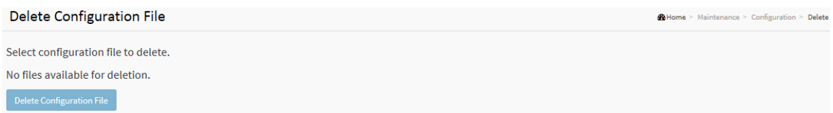
Figure 5-4.5: Delete Configuration
